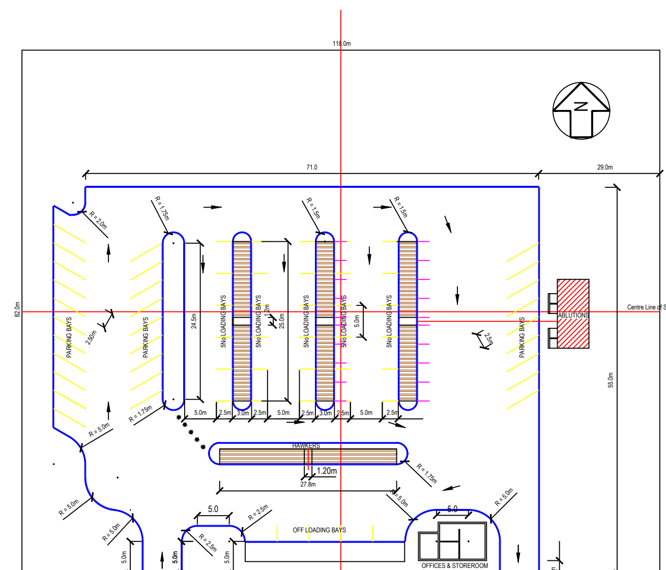
SITE LAYOUT
