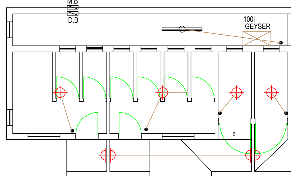
ELECTRICAL LAYOUT
