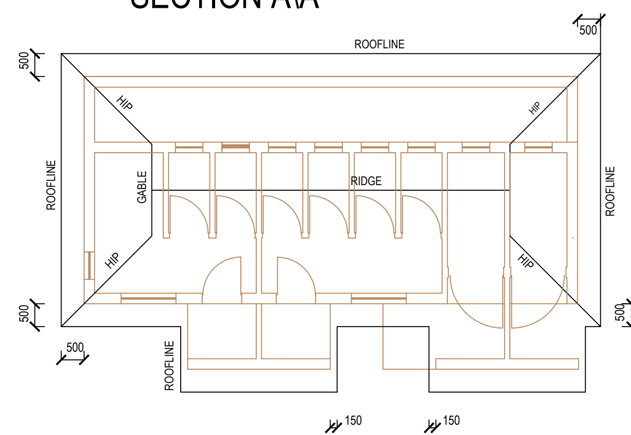
ROOF PLAN
